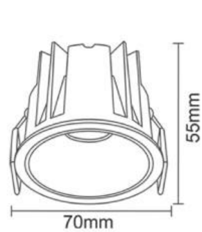
Cut-Out-60mm
