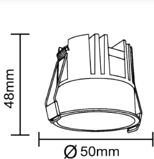
Dimension: D50*H48 Cut-out: Ø45
